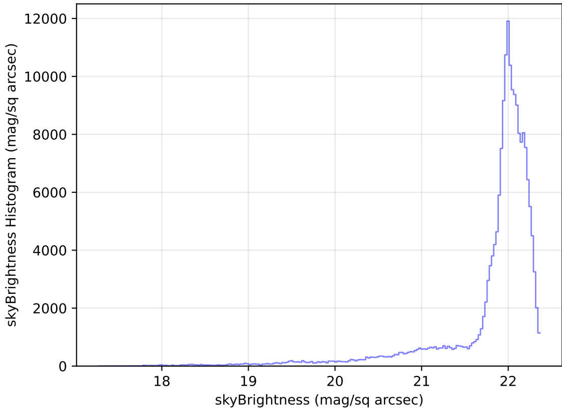
too_elab_r32_d2_giz_v3.4_10yrs WFD g band: skyBrightness Histogram
