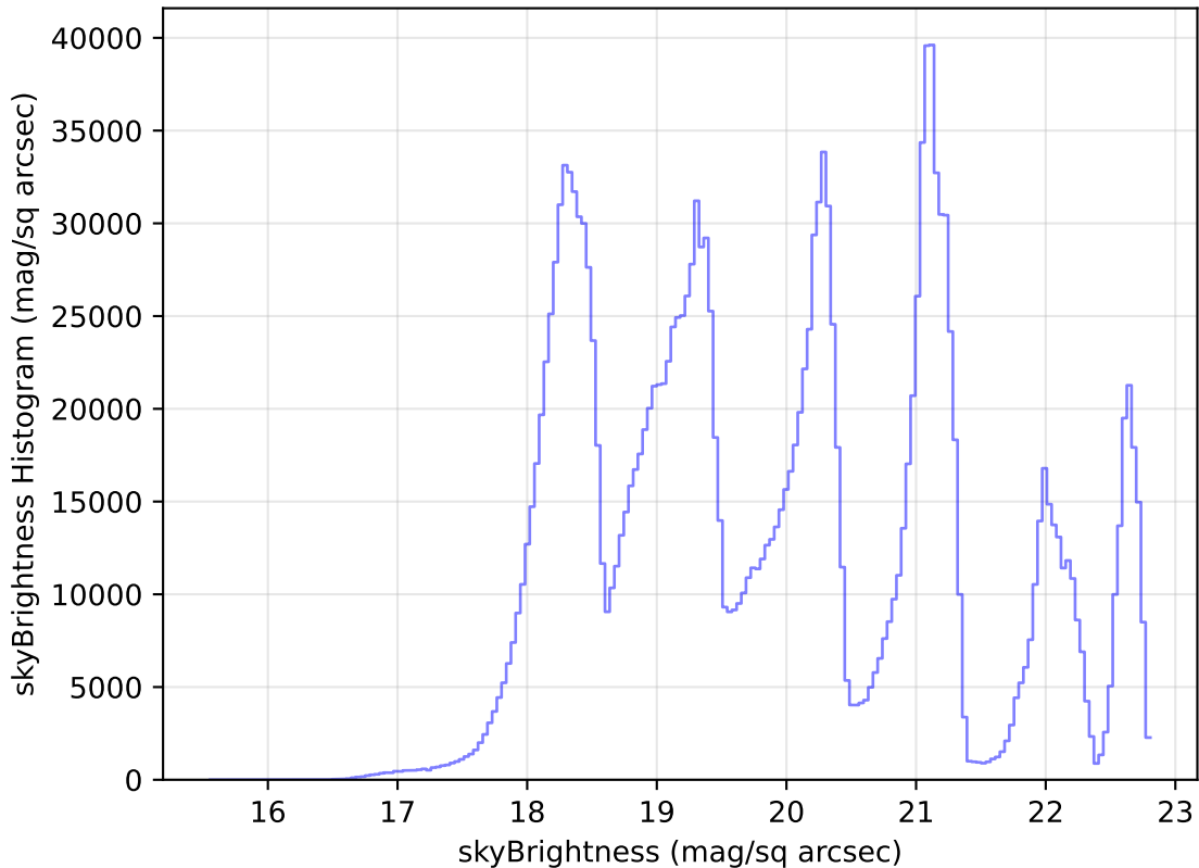
too_elab_r32_d2_giz_v3.4_10yrs WFD all bands: skyBrightness Histogram
