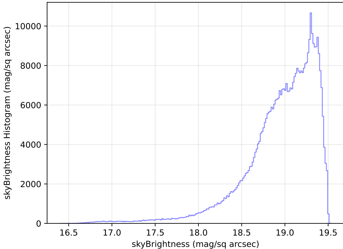
too_elab_r32_d2_giz_v3.4_10yrs All sky z band: skyBrightness Histogram
