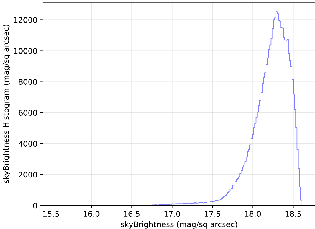
too_elab_r32_d2_giz_v3.4_10yrs All sky y band: skyBrightness Histogram
