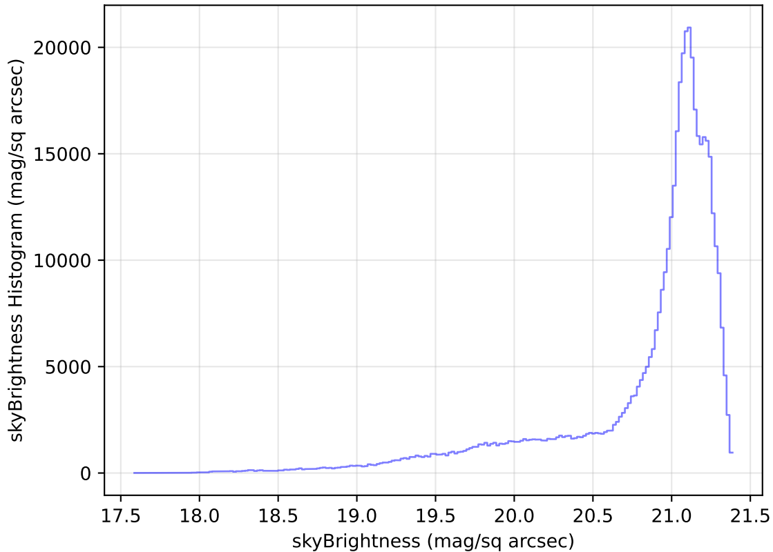
too_elab_r32_d2_giz_v3.4_10yrs All sky r band: skyBrightness Histogram
