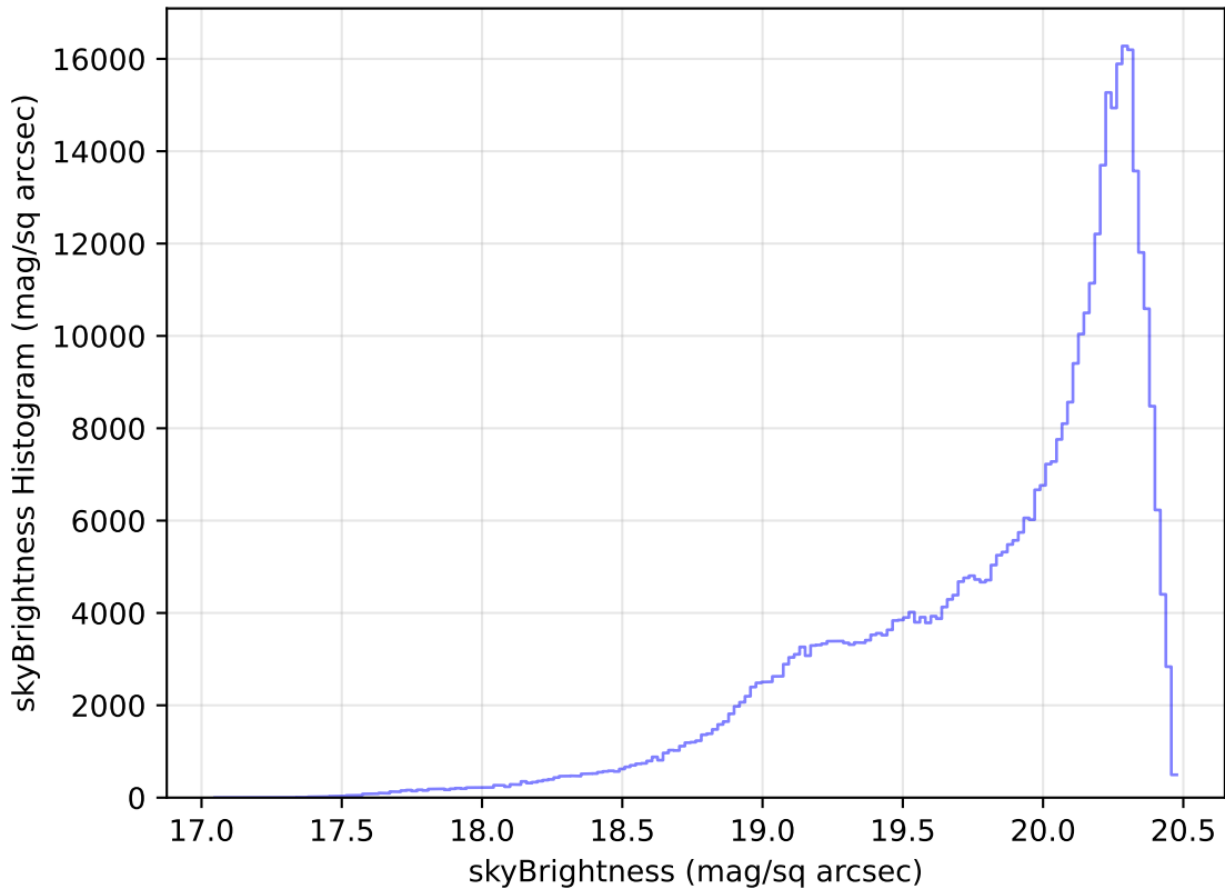
too_elab_r32_d2_giz_v3.4_10yrs All sky i band: skyBrightness Histogram
