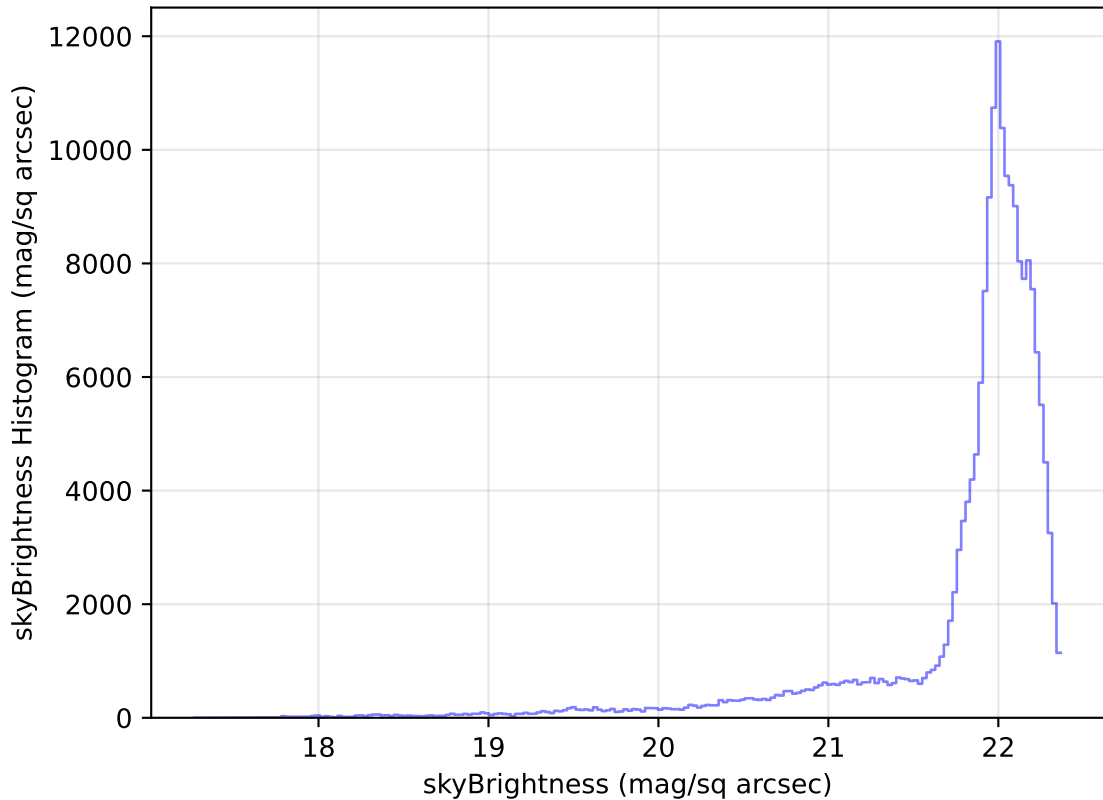
too_elab_r32_d2_giz_v3.4_10yrs All sky g band: skyBrightness Histogram
