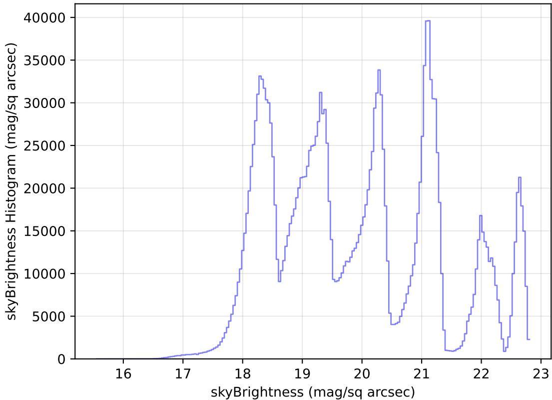
too_elab_r32_d2_giz_v3.4_10yrs All sky all bands: skyBrightness Histogram
