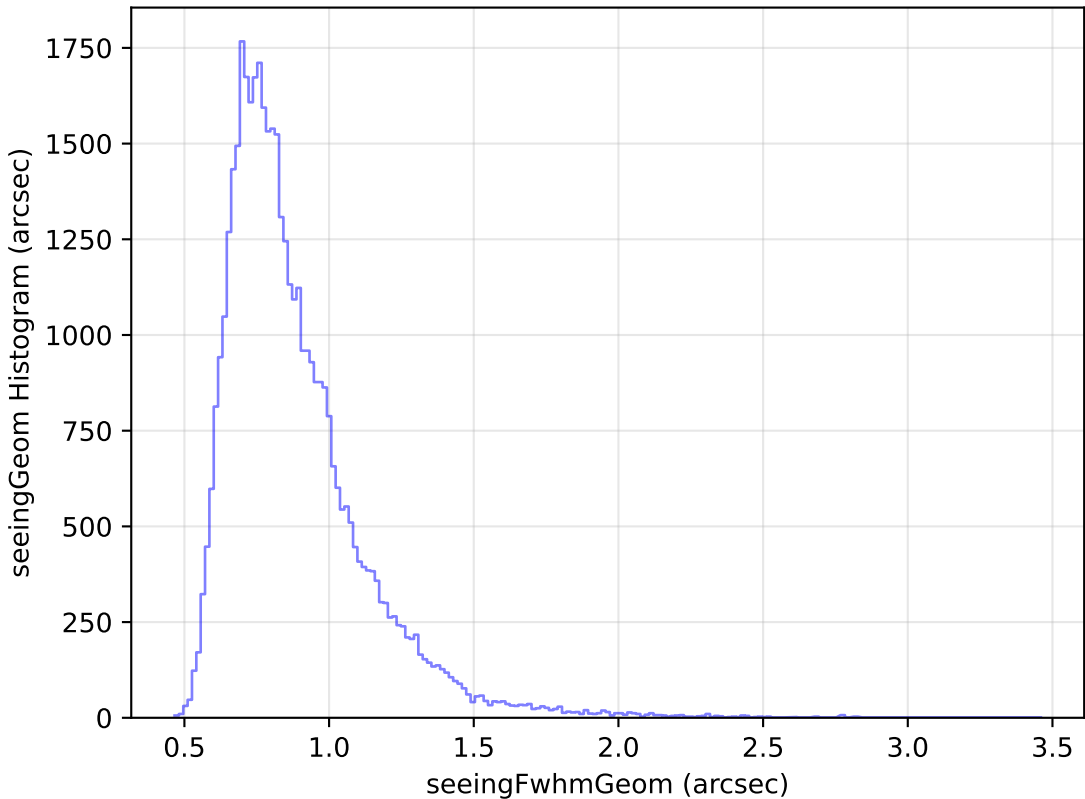
too_elab_r32_d2_giz_v3.4_10yrs Yr 1 z band: seeingGeom Histogram
