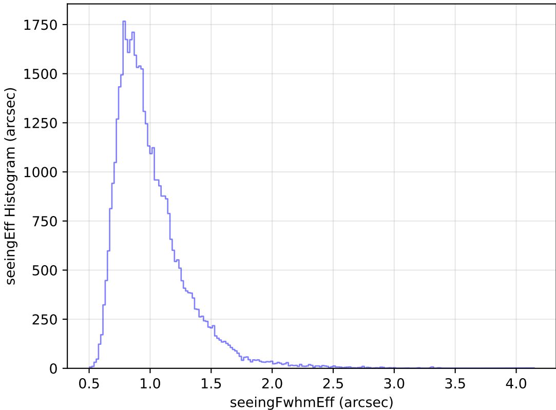
too_elab_r32_d2_giz_v3.4_10yrs Yr 1 z band: seeingEff Histogram
