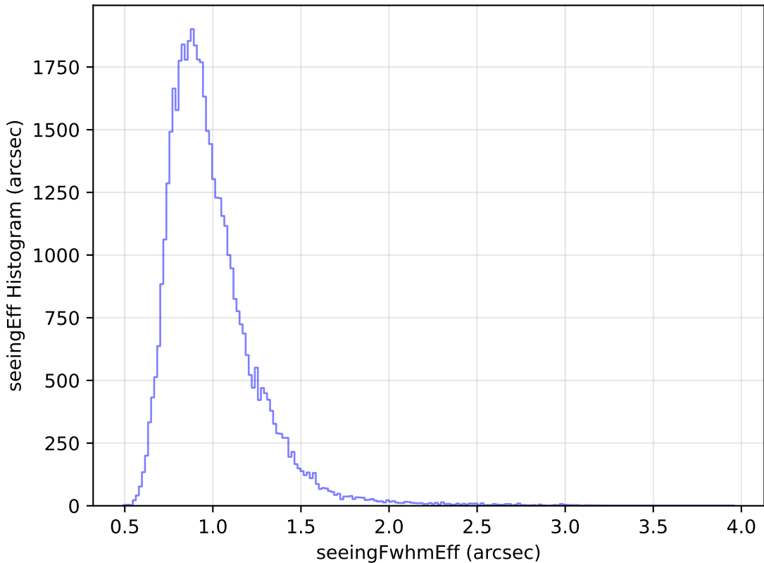
too_elab_r32_d2_giz_v3.4_10yrs Yr 1 y band: seeingEff Histogram
