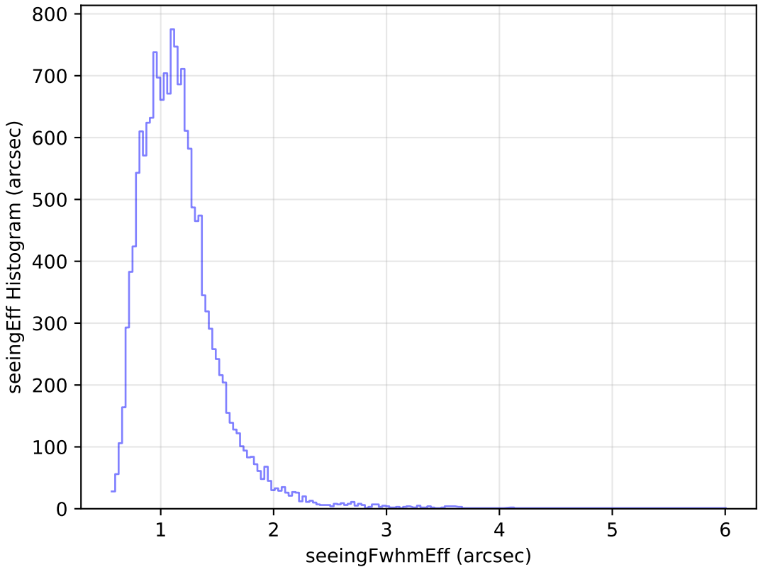
too_elab_r32_d2_giz_v3.4_10yrs Yr 1 u band: seeingEff Histogram
