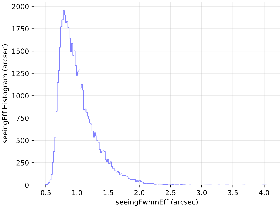
too_elab_r32_d2_giz_v3.4_10yrs Yr 1 r band: seeingEff Histogram
