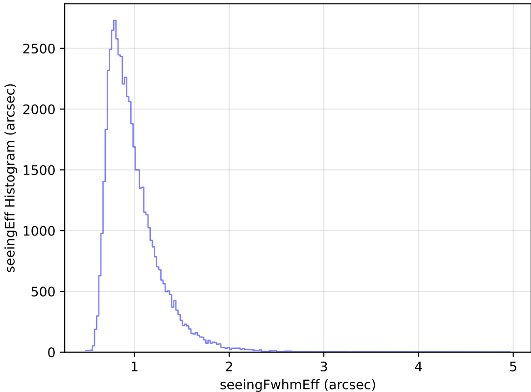
too_elab_r32_d2_giz_v3.4_10yrs Yr 1 i band: seeingEff Histogram
