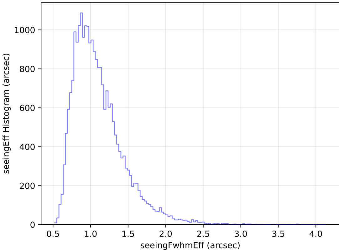
too_elab_r32_d2_giz_v3.4_10yrs Yr 1 g band: seeingEff Histogram
