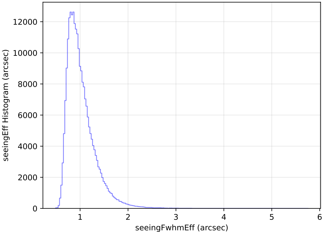
too_elab_r32_d2_giz_v3.4_10yrs Yr 1 all bands: seeingEff Histogram
