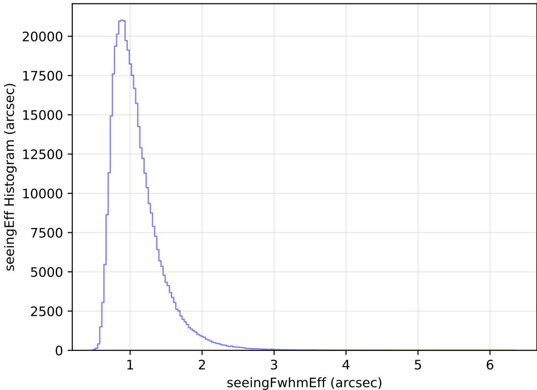
too_elab_r32_d2_giz_v3.4_10yrs WFD z band: seeingEff Histogram
