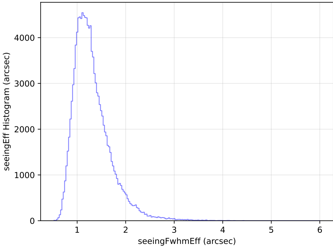
too_elab_r32_d2_giz_v3.4_10yrs WFD u band: seeingEff Histogram
