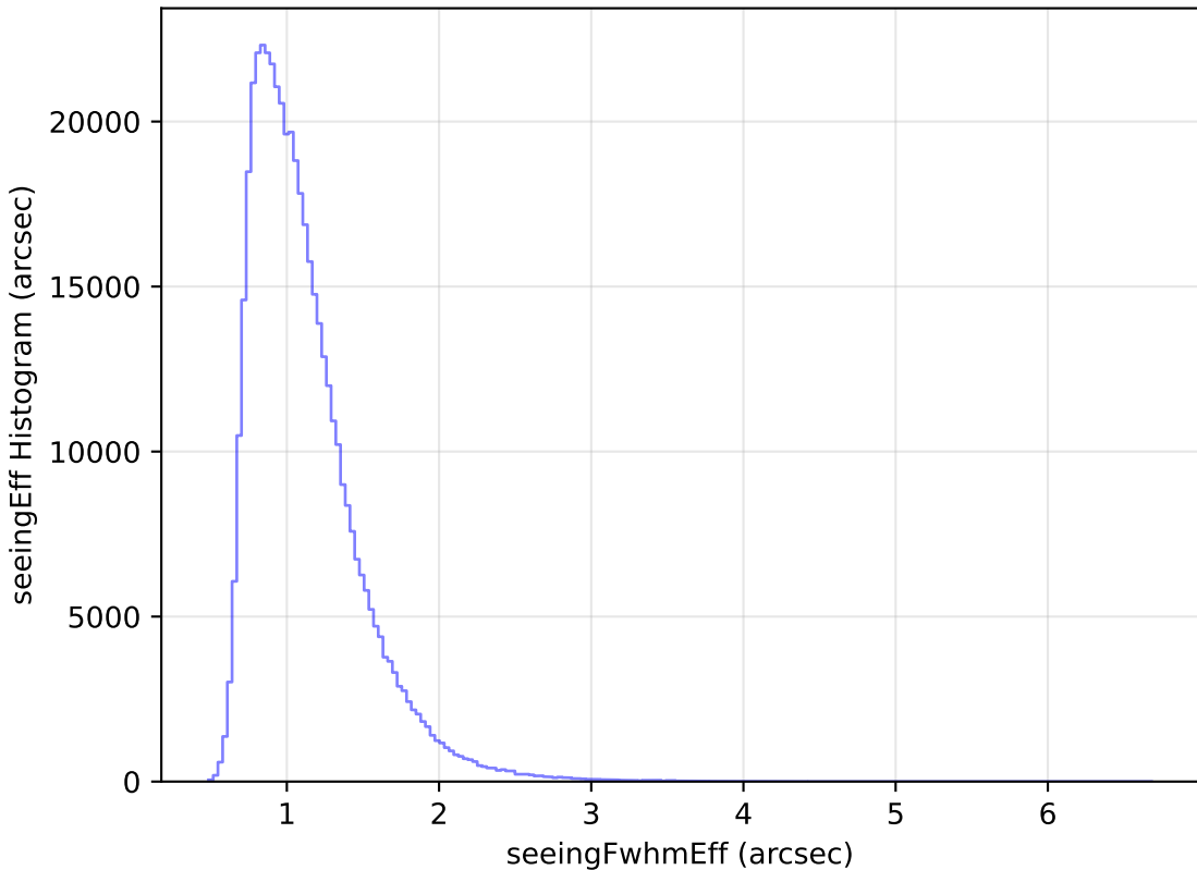
too_elab_r32_d2_giz_v3.4_10yrs WFD r band: seeingEff Histogram
