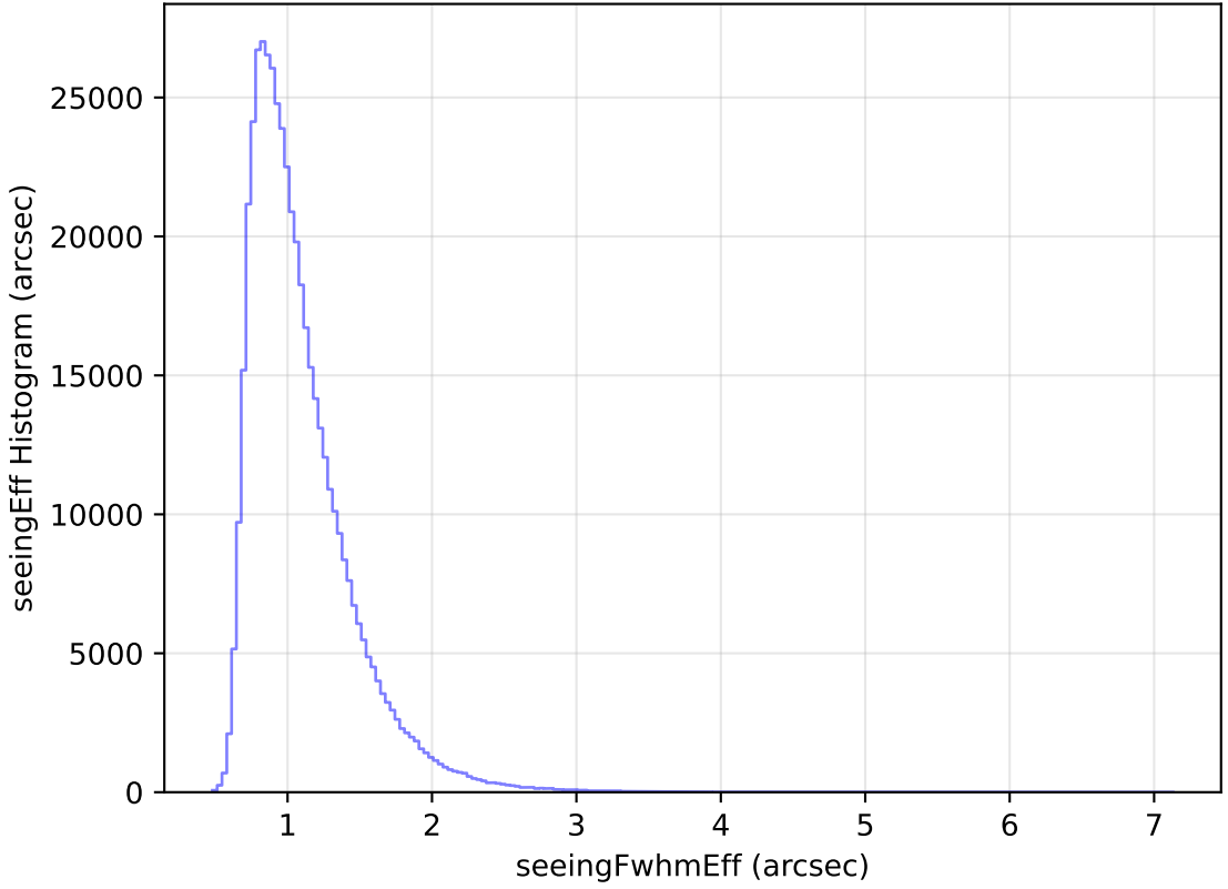
too_elab_r32_d2_giz_v3.4_10yrs WFD i band: seeingEff Histogram
