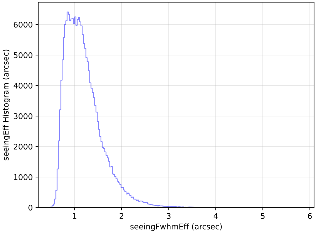
too_elab_r32_d2_giz_v3.4_10yrs WFD g band: seeingEff Histogram
