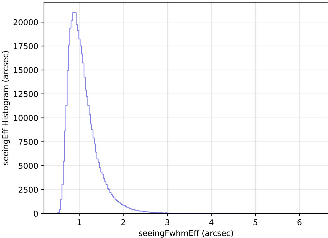
too_elab_r32_d2_giz_v3.4_10yrs All sky z band: seeingEff Histogram
