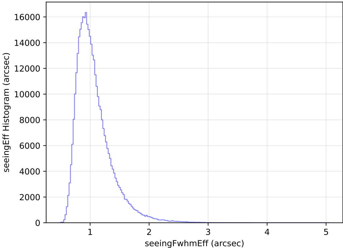
too_elab_r32_d2_giz_v3.4_10yrs All sky y band: seeingEff Histogram
