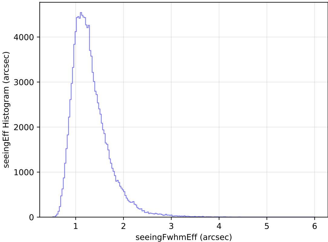
too_elab_r32_d2_giz_v3.4_10yrs All sky u band: seeingEff Histogram
