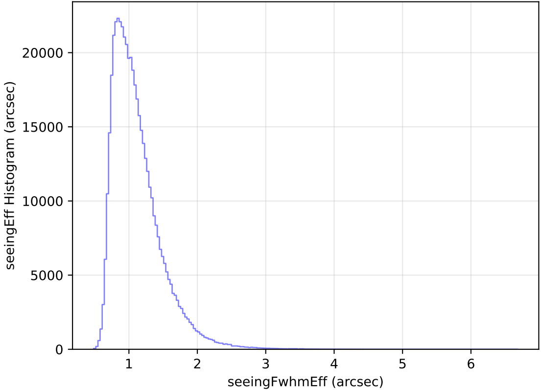
too_elab_r32_d2_giz_v3.4_10yrs All sky r band: seeingEff Histogram
