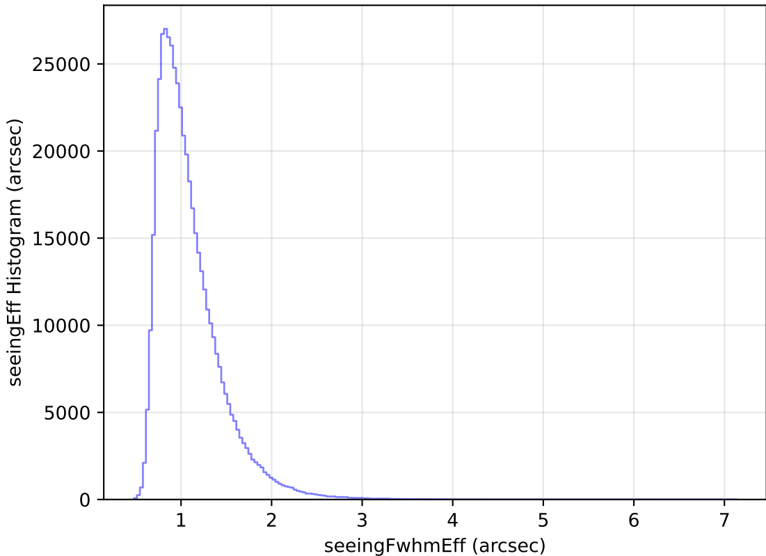
too_elab_r32_d2_giz_v3.4_10yrs All sky i band: seeingEff Histogram
