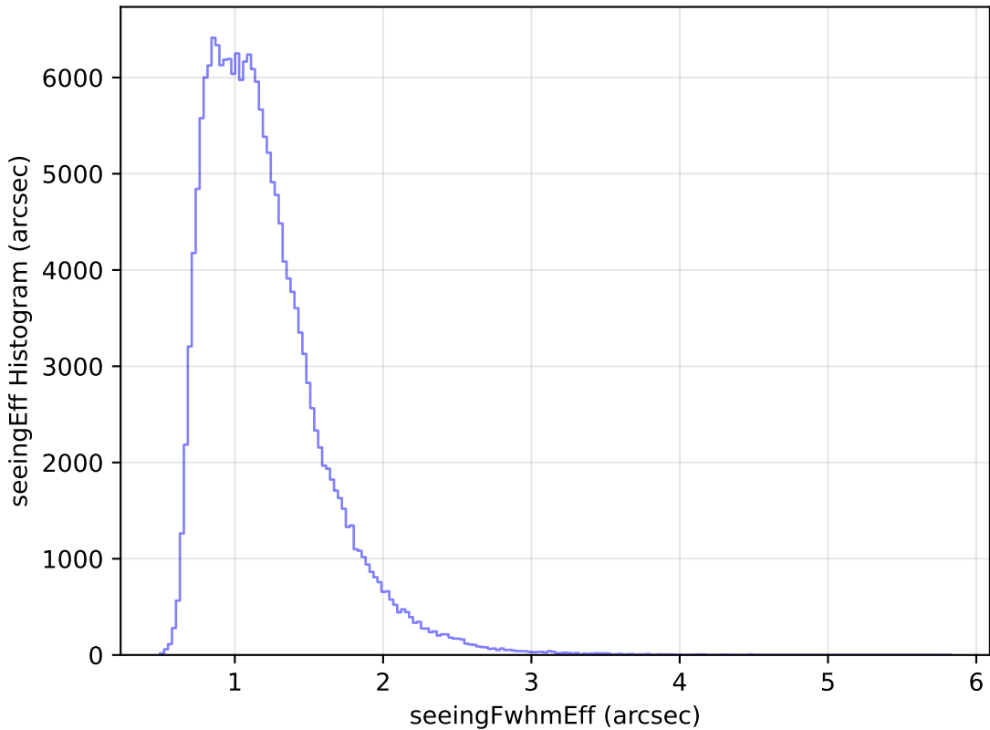
too_elab_r32_d2_giz_v3.4_10yrs All sky g band: seeingEff Histogram
