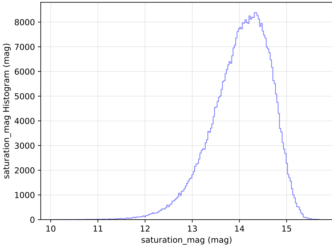
too_elab_r32_d2_giz_v3.4_10yrs WFD z band: saturation_mag Histogram
