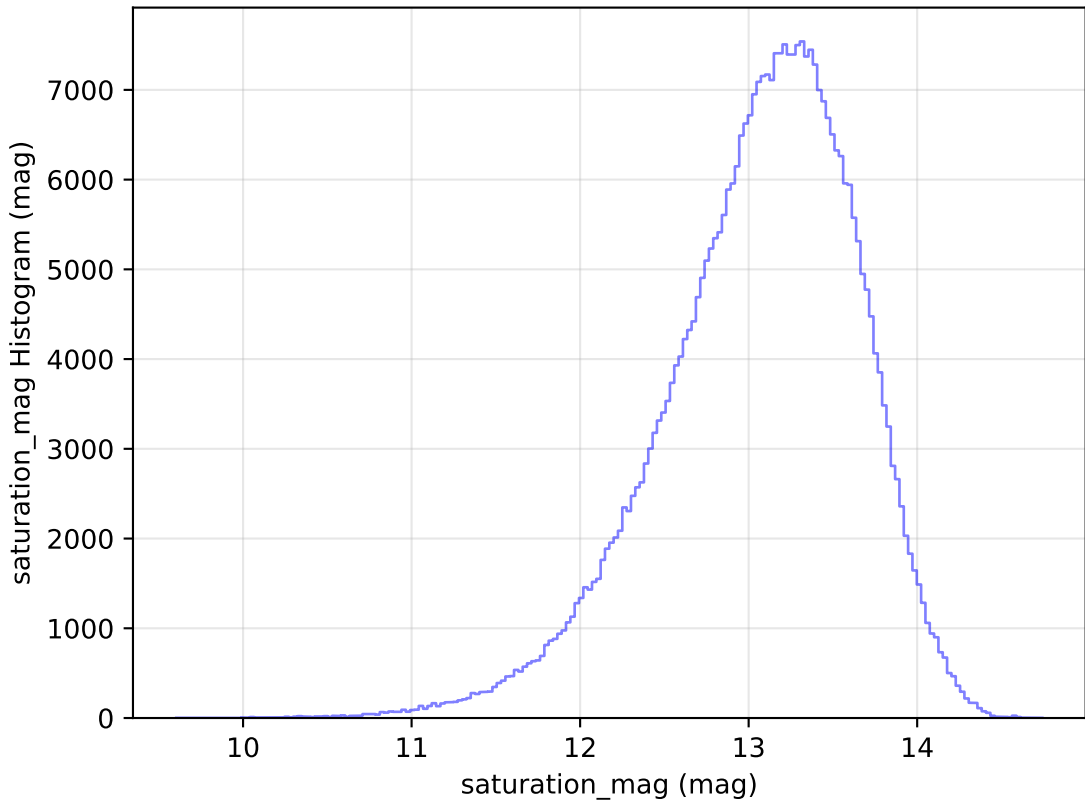
too_elab_r32_d2_giz_v3.4_10yrs WFD y band: saturation_mag Histogram
