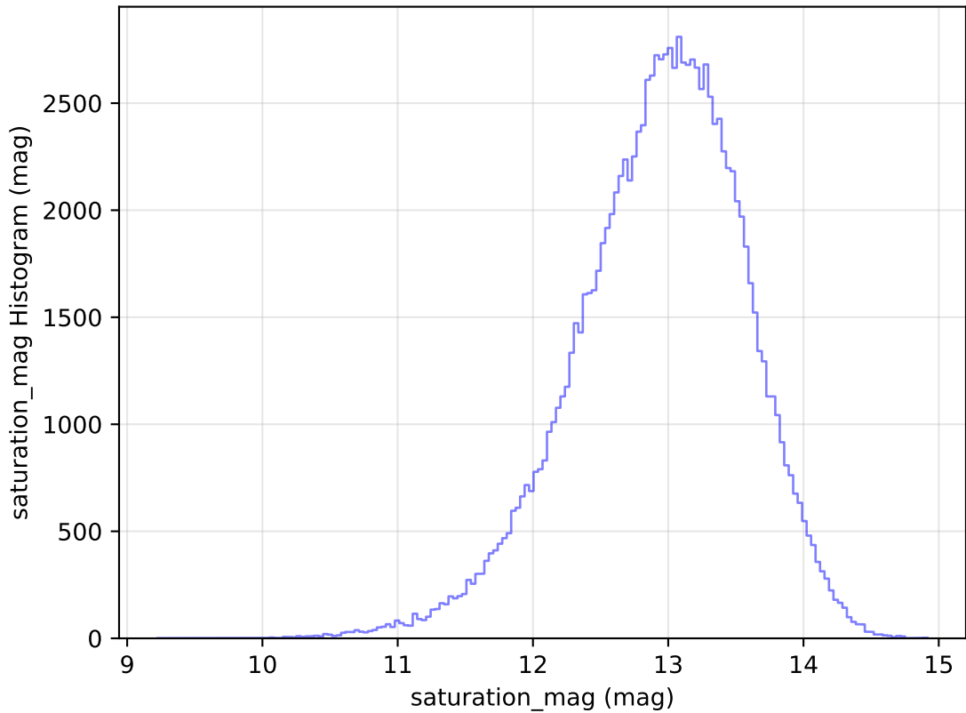
too_elab_r32_d2_giz_v3.4_10yrs WFD u band: saturation_mag Histogram
