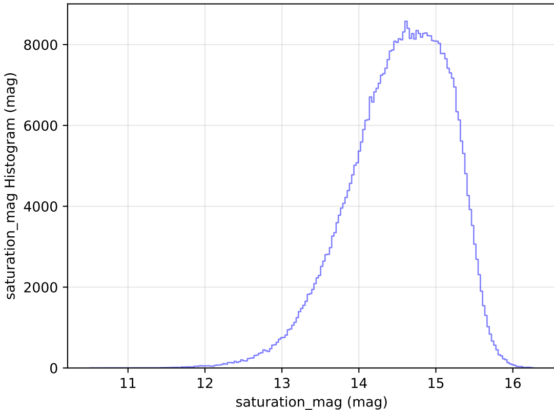
too_elab_r32_d2_giz_v3.4_10yrs WFD r band: saturation_mag Histogram
