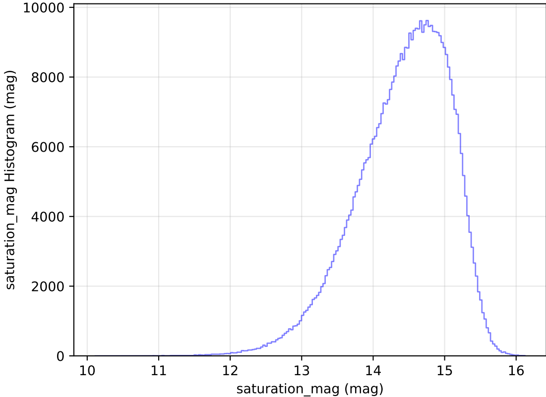
too_elab_r32_d2_giz_v3.4_10yrs WFD i band: saturation_mag Histogram
