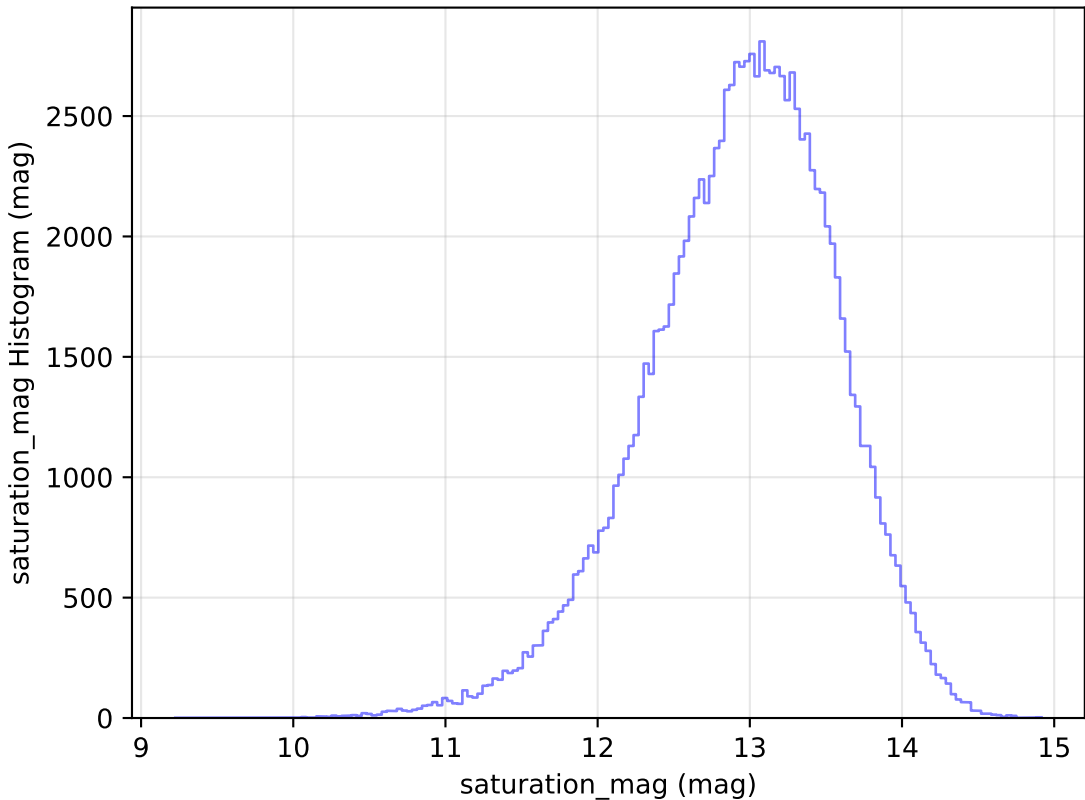
too_elab_r32_d2_giz_v3.4_10yrs All sky u band: saturation_mag Histogram
