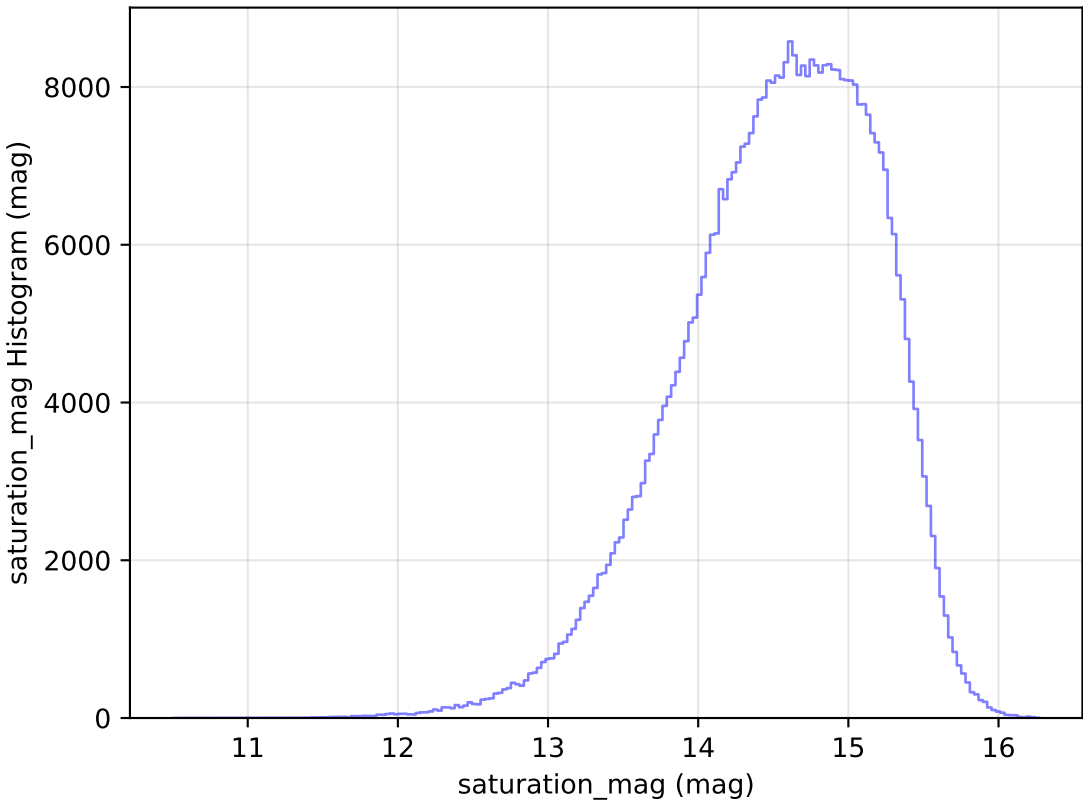
too_elab_r32_d2_giz_v3.4_10yrs All sky r band: saturation_mag Histogram
