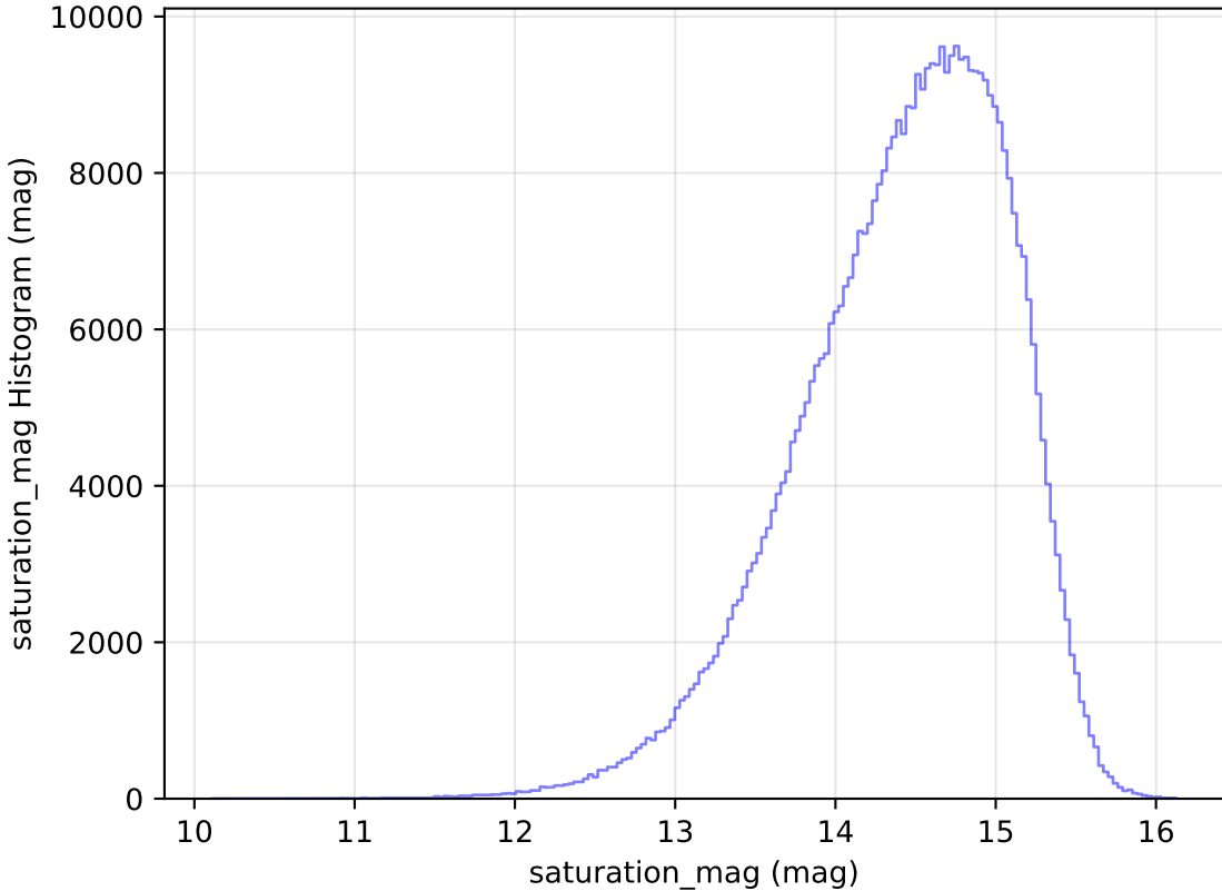
too_elab_r32_d2_giz_v3.4_10yrs All sky i band: saturation_mag Histogram
