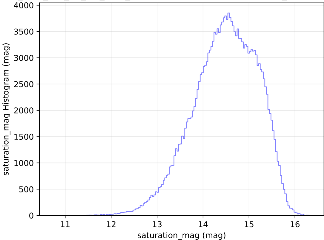
too_elab_r32_d2_giz_v3.4_10yrs All sky g band: saturation_mag Histogram
