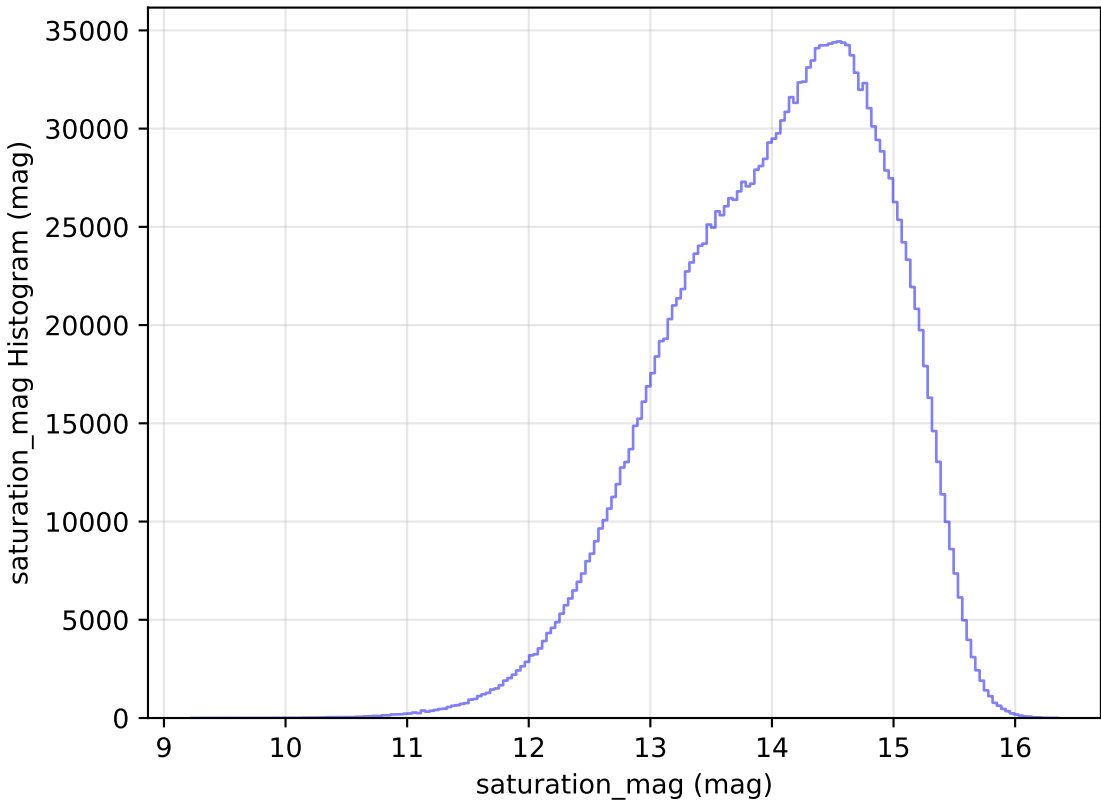
too_elab_r32_d2_giz_v3.4_10yrs All sky all bands: saturation_mag Histogram
