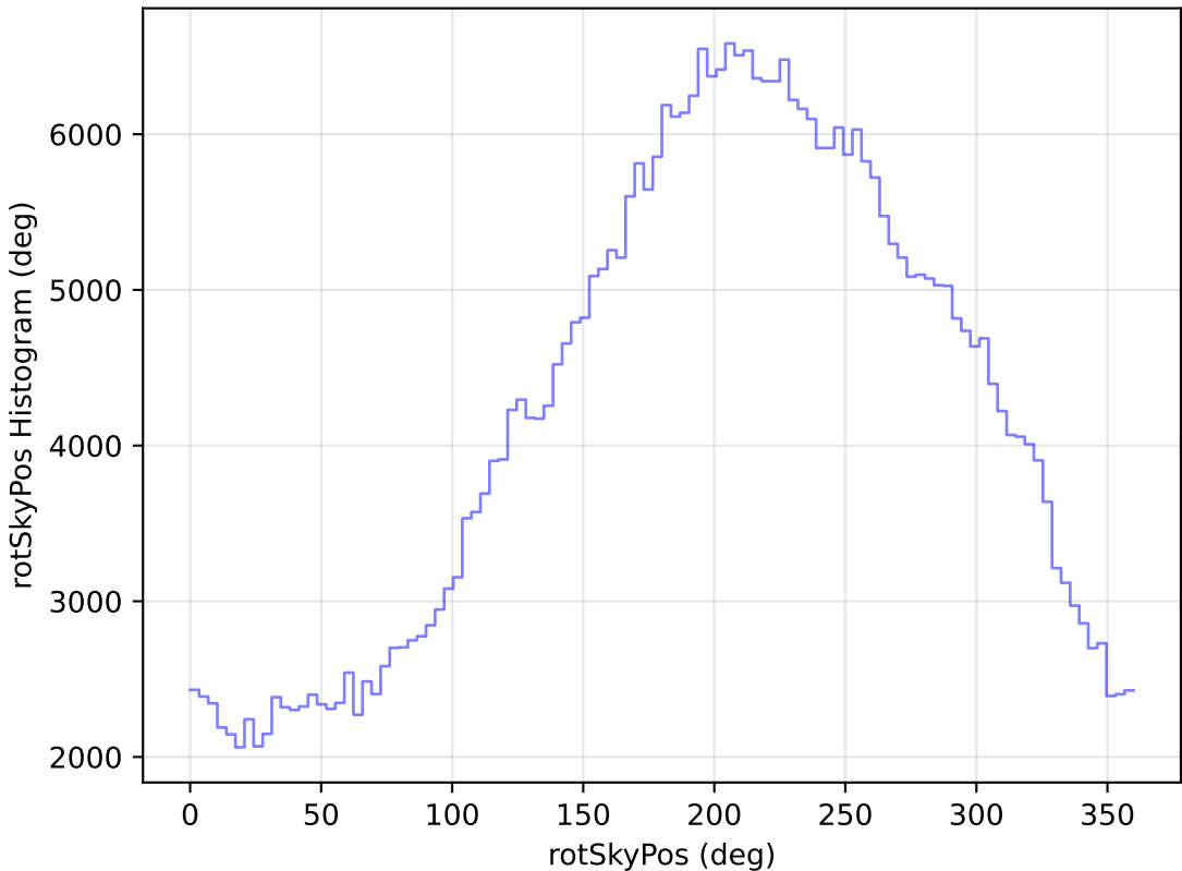
too_elab_r32_d2_giz_v3.4_10yrs WFD z band: rotSkyPos Histogram
