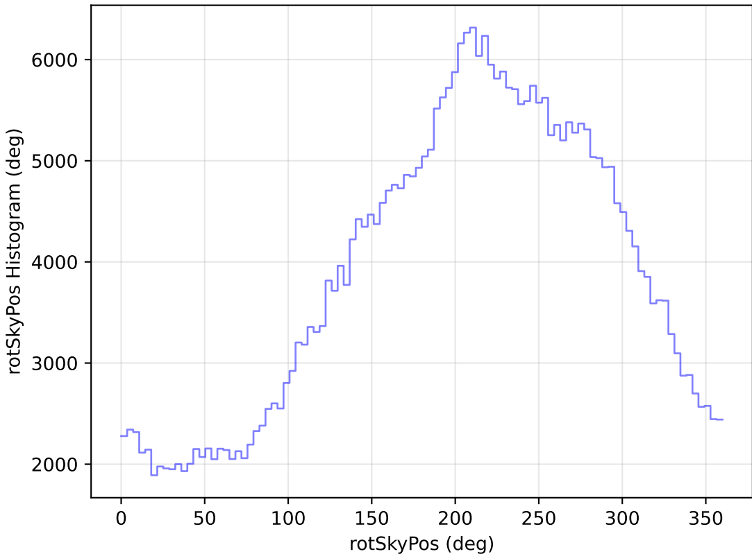
too_elab_r32_d2_giz_v3.4_10yrs WFD y band: rotSkyPos Histogram
