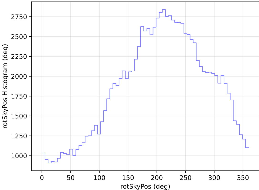
too_elab_r32_d2_giz_v3.4_10yrs WFD u band: rotSkyPos Histogram
