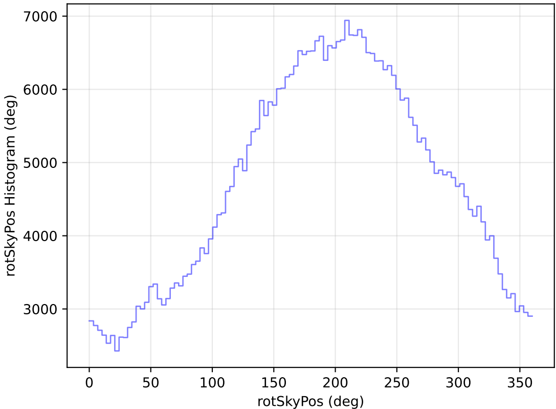
too_elab_r32_d2_giz_v3.4_10yrs WFD r band: rotSkyPos Histogram
