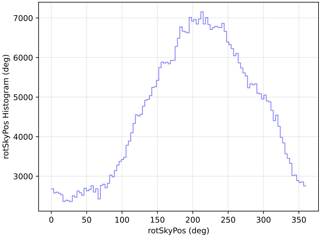
too_elab_r32_d2_giz_v3.4_10yrs WFD i band: rotSkyPos Histogram
