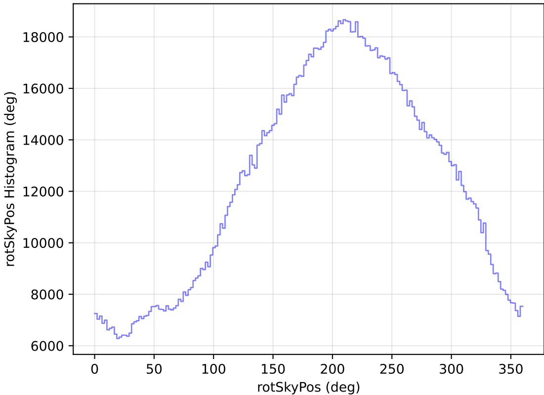
too_elab_r32_d2_giz_v3.4_10yrs WFD all bands: rotSkyPos Histogram
