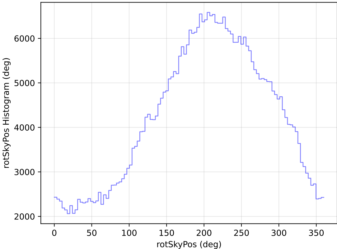
too_elab_r32_d2_giz_v3.4_10yrs All sky z band: rotSkyPos Histogram
