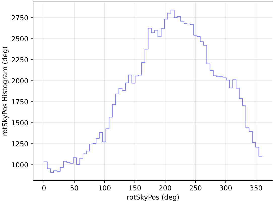
too_elab_r32_d2_giz_v3.4_10yrs All sky u band: rotSkyPos Histogram
