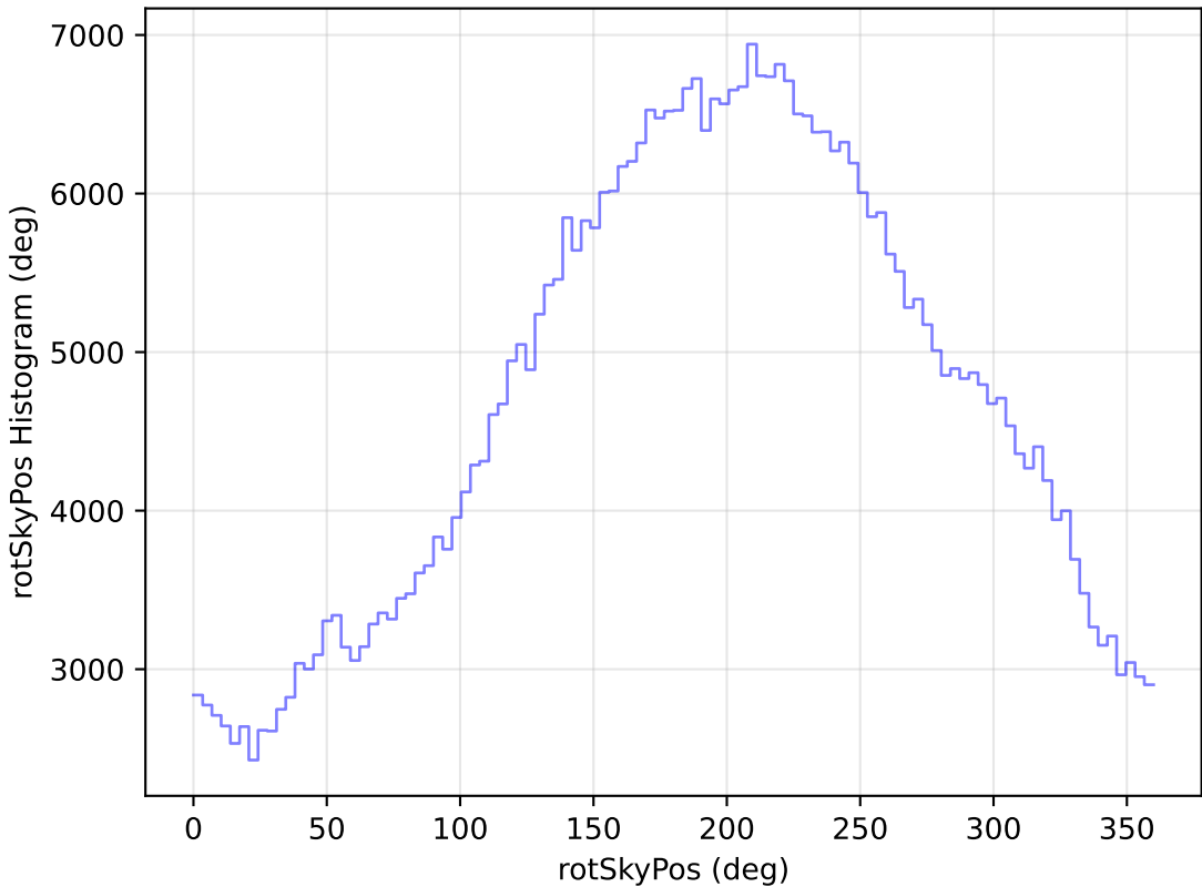
too_elab_r32_d2_giz_v3.4_10yrs All sky r band: rotSkyPos Histogram
