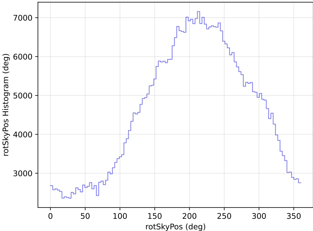
too_elab_r32_d2_giz_v3.4_10yrs All sky i band: rotSkyPos Histogram
