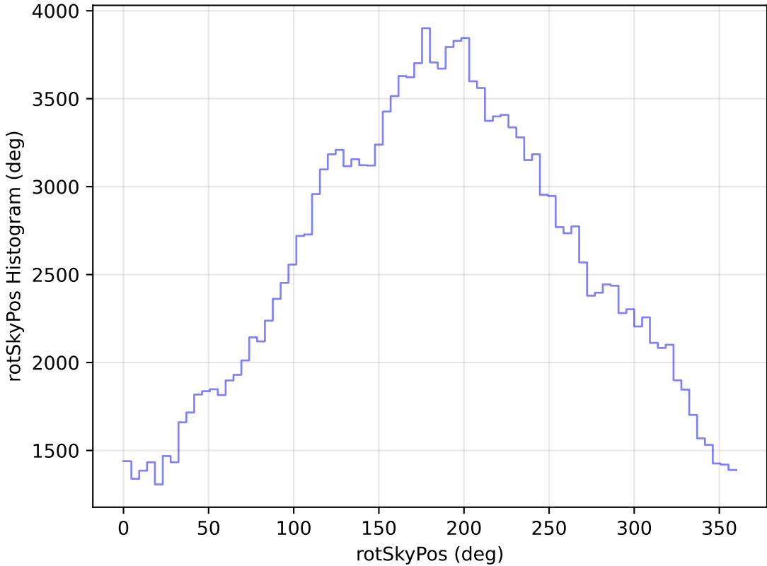
too_elab_r32_d2_giz_v3.4_10yrs All sky g band: rotSkyPos Histogram
