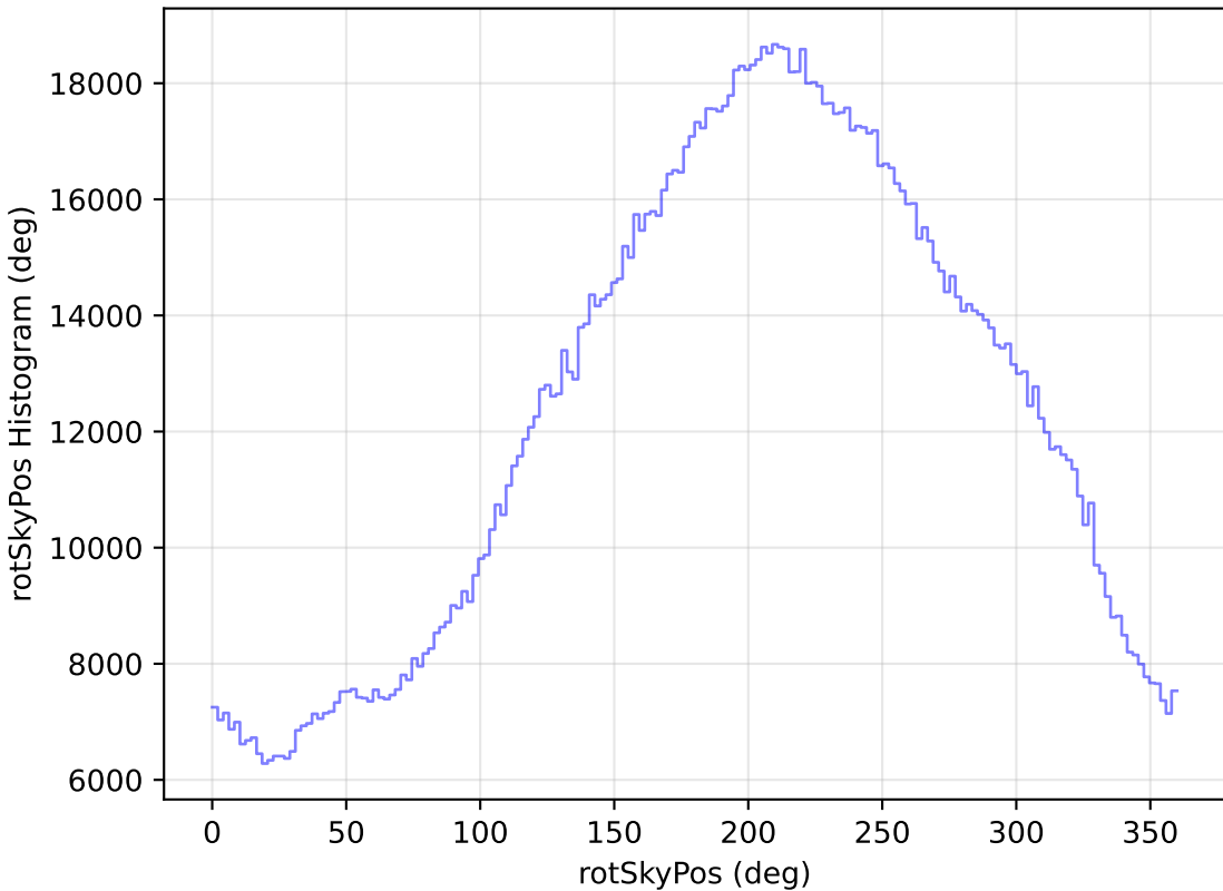
too_elab_r32_d2_giz_v3.4_10yrs All sky all bands: rotSkyPos Histogram
