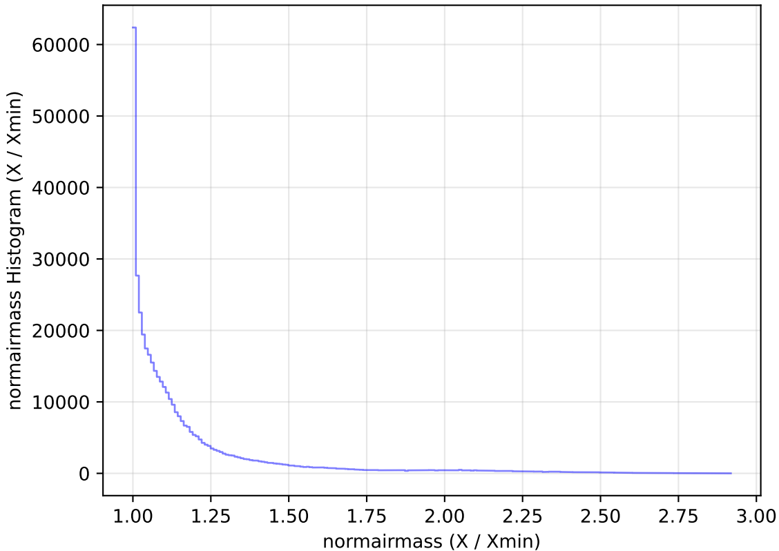
too_elab_r32_d2_giz_v3.4_10yrs WFD z band: normairmass Histogram
